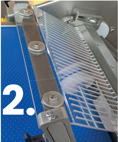
2. The “piano” system (patented by VARLET) ensures a firm grip on the product right from the start, to remove the skin from skate wings or flat fishes.
